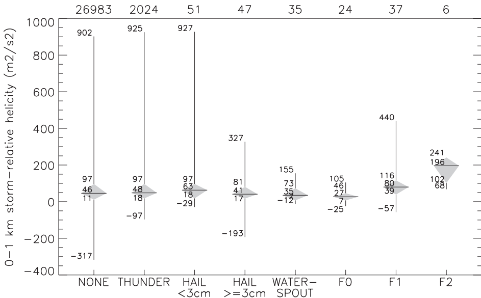
Fig. 8. As Fig. 2, but for 0–1 km storm-relative helicity.
